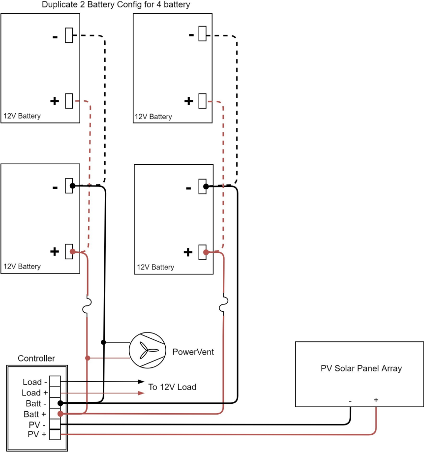
RemotePro 12V Wiring Diagram
