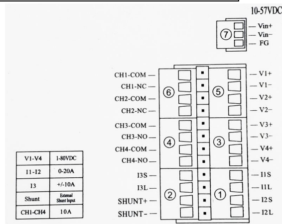
TPDIN® Connector Pinout
